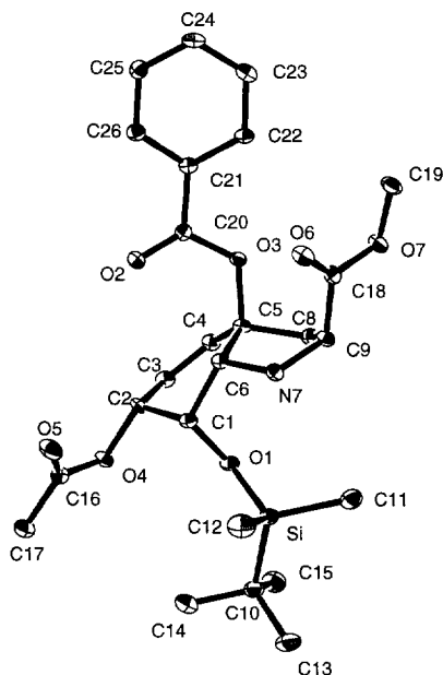
Figure 2. Ortep drawing of crystal structure of 14 .
