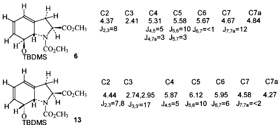
Figure 1. Chemical shift and coupling constants for compounds 6 and 13 .
